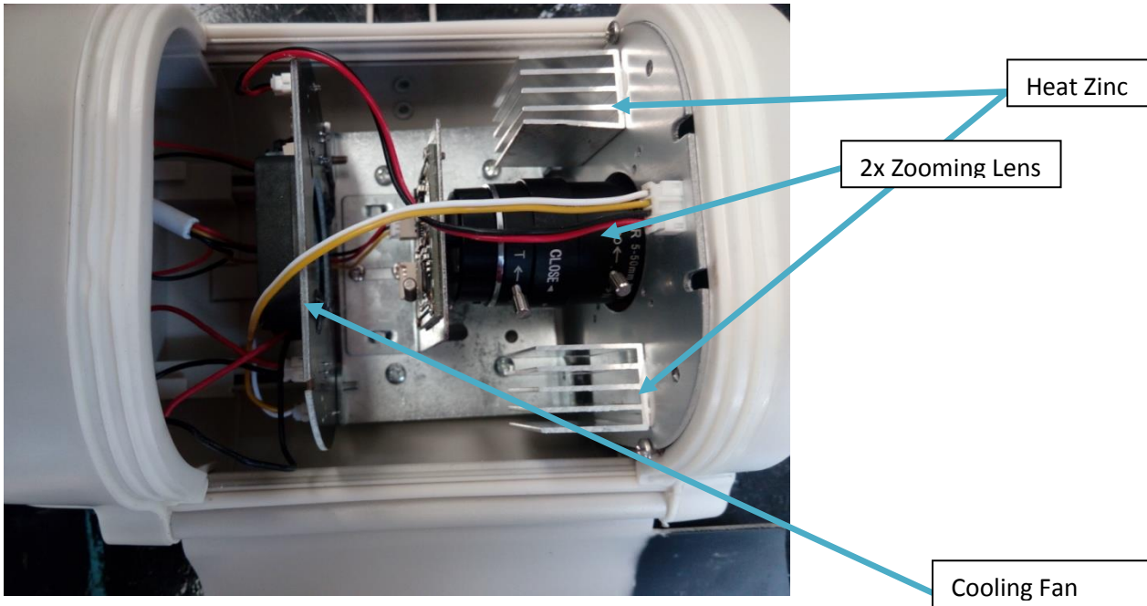
FRONT VIEW
